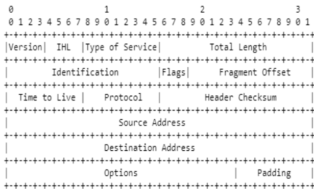
Figure (1) IPv4 protocol header according to RFC 791
